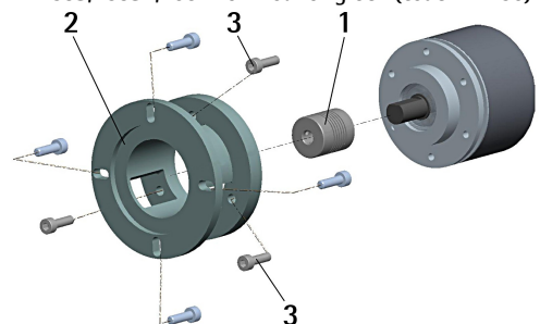
I58S, I58SK, I65 with mounting bell (code PF4256)
