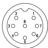
M12 8-pin connector A coding Male frontal side
